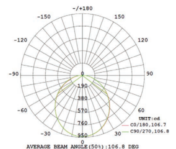
Luminous intensity distribution LED only
